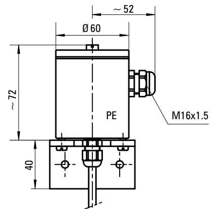
Bemaßung in mm / Dimensioning in mm
