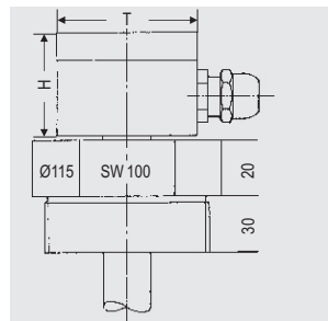
Tip / Type RPV-VPV-A3"-AA(PO) = cev zalepljena Pipe glued RPP-VPP-A3"-AA(PO) = cev pod sponom Screw pipe RPT-VPT-A3"-AA(PO) = cev pod sponom Pipe clamped RPE-VPE-A3"-AA(PO) = cev zavarena Pipe welded
