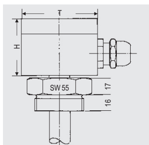
Tip / Type RMS-VMS-A1½"-AA(PO) = cev zavarena Pipe brazed RVA-VMS-A1½"-AA(PO) = cev pod sponom Screw pipe RMS-VVA-A1½"-AA(PO) = cev pod sponom Screw pipe RVA-VVA-A1½"-AA(PO) = cev zalemljena Pipe welded
