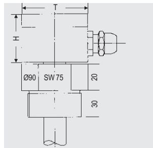
Tip / Type RPV-VPV-A2"-AA(PO) = cev zalepljena Pipe glued RPP-VPP-A2"-AA(PO) = cev zavrnuta Screw pipe RPT-VPT-A2"-AA(PO) = cev pod sponom Pipe clamped RPE-VPE-A2"-AA(PO) = cev zavarena Pipe welded
