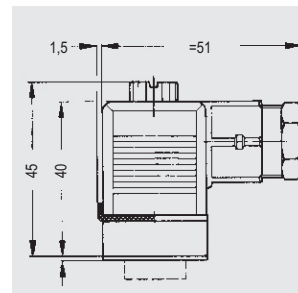
Utikac / Connection Plug
