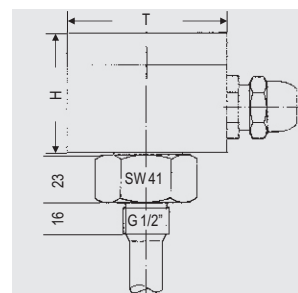
Tip / Type RMS-VMS-A½"-AA(PO) = cev zavarena Pipe brazed RVA-VMS-A½"-AA(PO) = cev pod sponom Screw pipe RMS-VVA-A½"-AA(PO) = cev pod sponom Screw pipe RVA-VVA-A½"-AA(PO) = cev zalemljena Pipe welded
