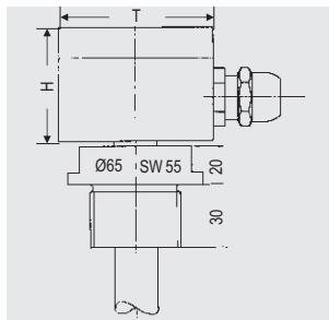
Tip / Type RMS-VPP(VPE)-A1½"-AA(PO) = cev zavarena Screw pipe RVA-VPP(VPE)-A1½"-AA(PO) = cev zavarena Screw pipe
